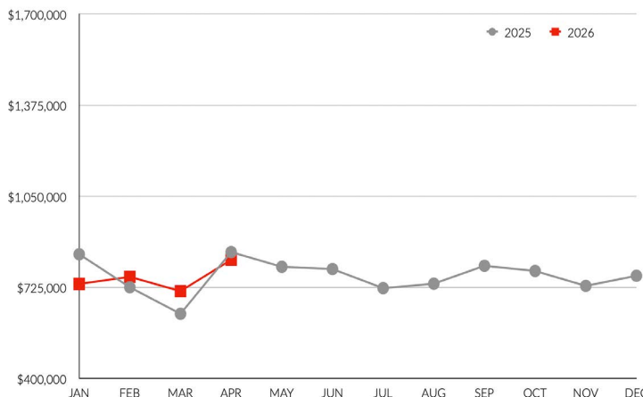
Month-Over-Month 2025 vs. 2026
