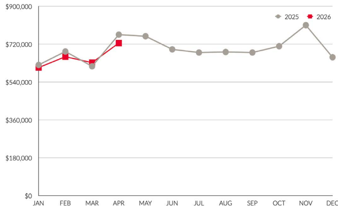
Month-Over-Month 2025 vs. 2026
